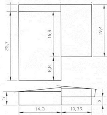
main dimensions of the building
